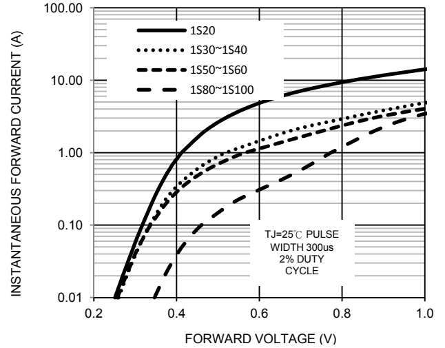
FIG. 2-TYPICAL FORWARD CHARACTERISTICS
