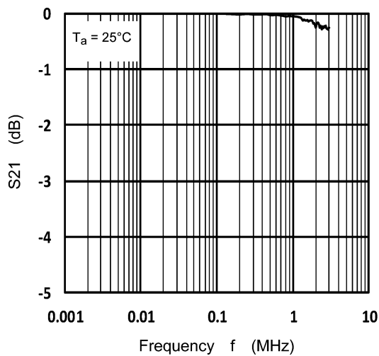
図 10.1 S_{21} - f
