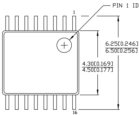
Figure 11. 16-Pin TSSOP 4.40 mm Body Z16.173
