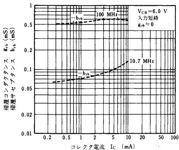
REVERSE TRANSFER ADMITTANCE ( y_{rb} ) vs. COLLECTOR CURRENT
