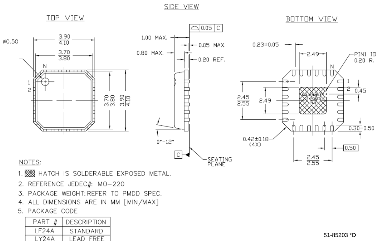
Figure 19. 24-Pin (4 × 4) QFN
