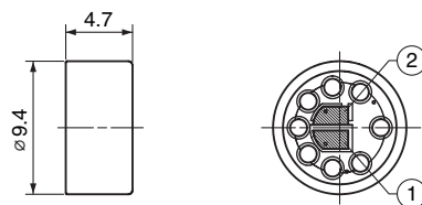
Lead Wire Type
