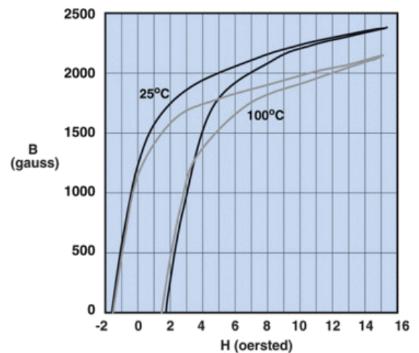
Hysteresis Loop
