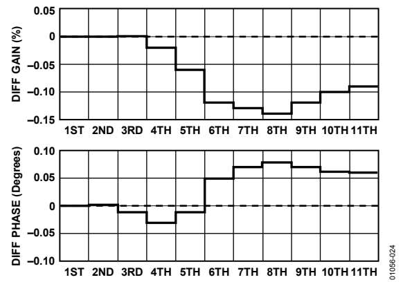
図24. 微分ゲインと微分位相、V S = ±5 V、R L = 1 kΩ
