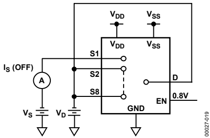
図19. I_S (OFF)
