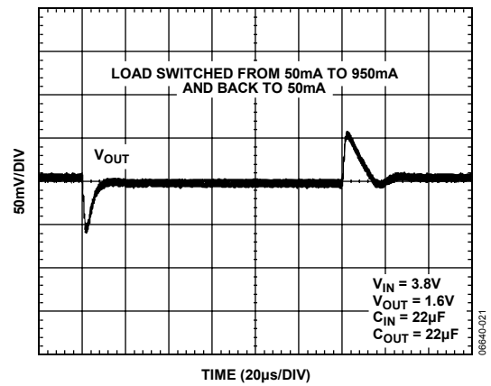
図 20. 負荷過渡応答 ( C_{IN} = 22 \mu\text{F} 、 C_{OUT} = 22 \mu\text{F} )
