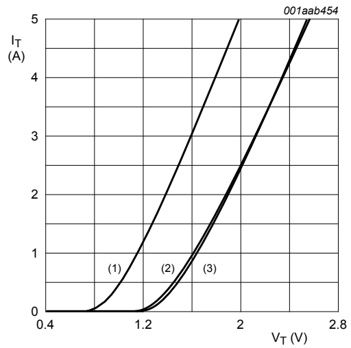
Fig. 10. On-state current as a function of on-state voltage V o = 1.067 V; R s = 0.187 Ω (1) T j = 125 °C; typical values (2) T j = 125 °C; maximum values (3) T j = 25 °C; maximum values
