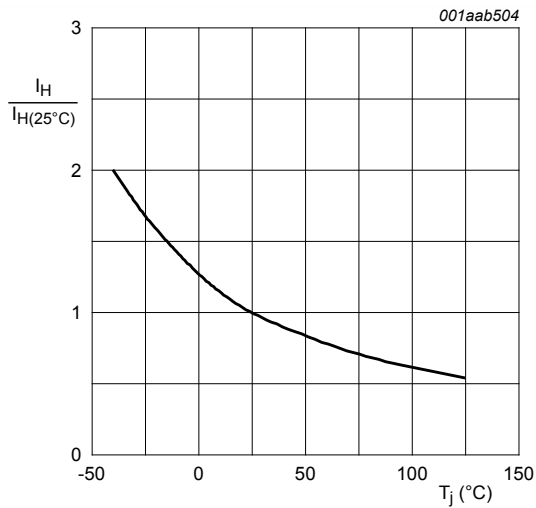
Fig. 9. Normalized holding current as a function of junction temperature R GK = 1 kΩ
