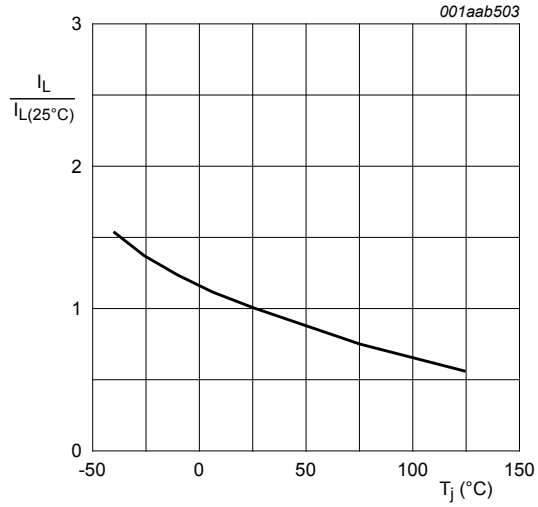
Fig. 8. Normalized latching current as a function of junction temperature R GK = 1 kΩ
