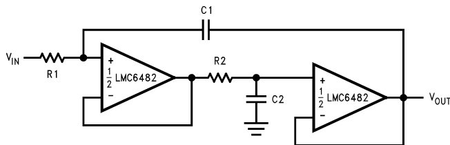
Figure 77. Rail-To-Rail Single Supply Low Pass Filter
