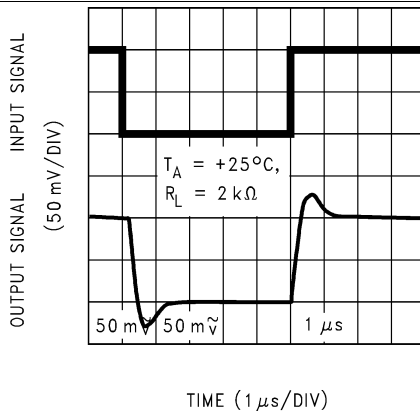
Figure 39. Noninverting Small Signal Pulse Response
