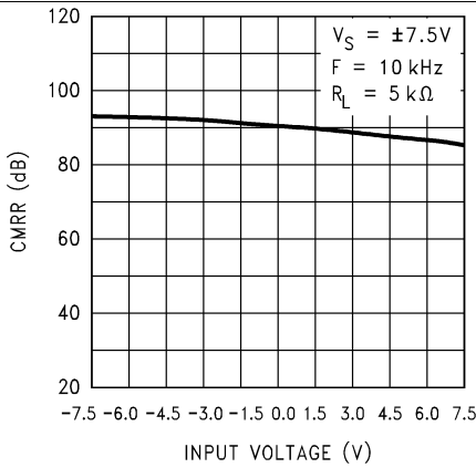
Figure 19. CMRR vs. Input Voltage
