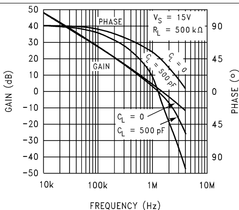
Figure 30. Gain and Phase vs. Capacitive Load
