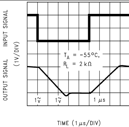
Figure 37. Noninverting Large Signal Pulse Response
