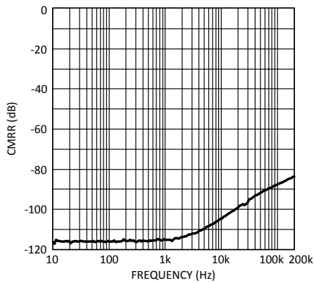
Figure 89. Cmrr vs Frequency V_{CC} = 15V , V_{EE} = -15V R_L = 10k\Omega
