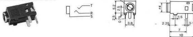
No.MJ-2-348A0 (φ2.5) With Metal Sleeve No.MJ-2-348B0 (φ2.5) Without Metal Sleeve SUB-MINIATURE STEREO JACK
