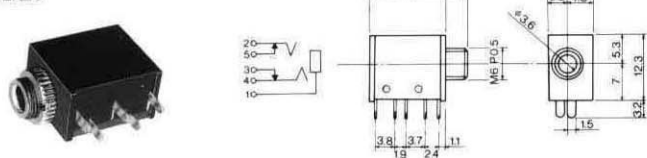
No.MJ-354W-SG (φ3.5) STEREO
