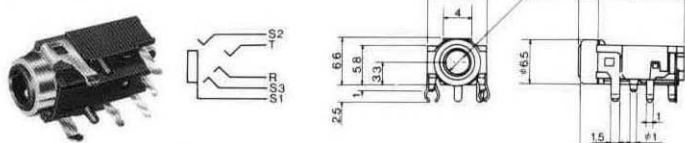
No.M03-428 (φ3.5) 6-CONDUCTOR
