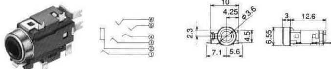
No.M03-721C0 (φ3.5) 6-CONDUCTOR
