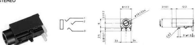
No.M03-681A0 (φ3.5) STEREO
