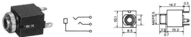
No.MJ-355W (φ3.5) CHASSIS MTG. STEREO JACK
