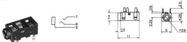
No.MJ-A18 (φ2.5) STEREO
