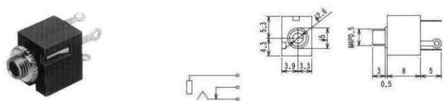
No.M03-681A0 (φ3.5) STEREO
