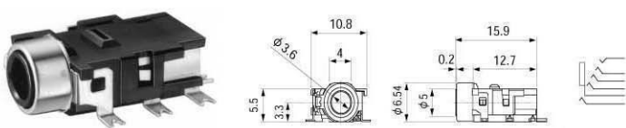
No.MJ-354W-S2 3.5MM STEREO JACK FOR P.C. W/SHIELD HOUSING
