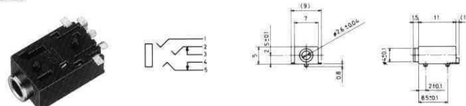
No.M02-641A0 (φ2.5) STEREO
