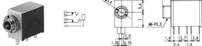
No.MJ-355 (φ3.5) MONO
