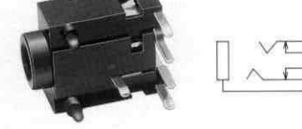
No.MJ-3235 (φ3.5) MONO
