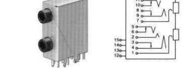
No.MJ-653 3.5MM DOUBLE STEREO JACK FOR P.C. W/FULL SHIELD HOUSING
