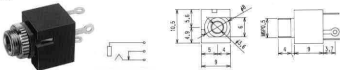
No.MJ-355 (φ3.5) MONO
