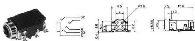
No.MX-385AGM (φ3.5) 5-CONDUCTOR
