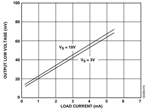
Figure 15. Output Low Voltage to Supply Rail vs. Load Current
