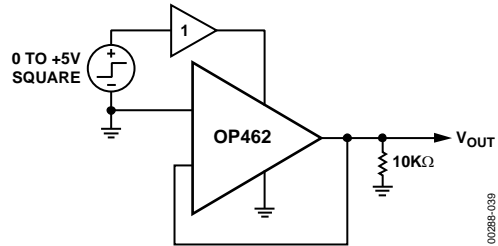
Figure 38. Test Circuit for Power-On Settling Time
