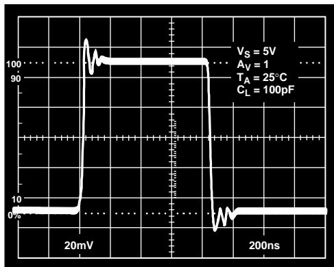
Figure 30. Small Signal Transient Response
