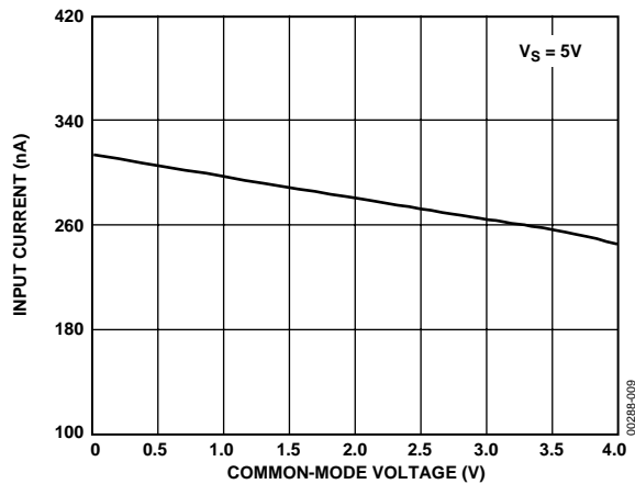
Figure 8. OP462 Input Bias Current vs. Common-Mode Voltage
