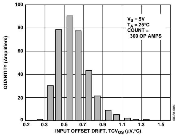
Figure 7. OP462 Input Offset Voltage Drift (TCVos)
