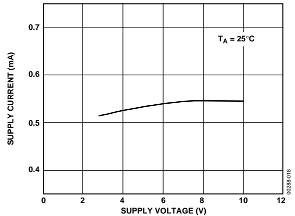
Figure 17. OP462 Supply Current/Amplifier vs. Supply Voltage
