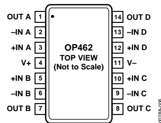
Figure 5. 14-Lead TSSOP (RU Suffix)
