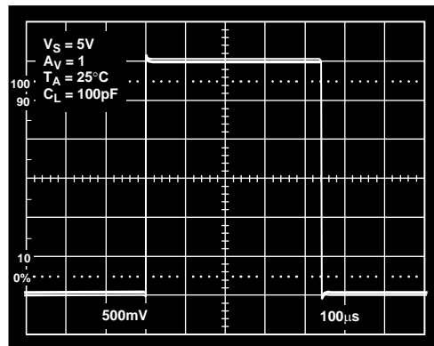
Figure 31. Large Signal Transient Response
