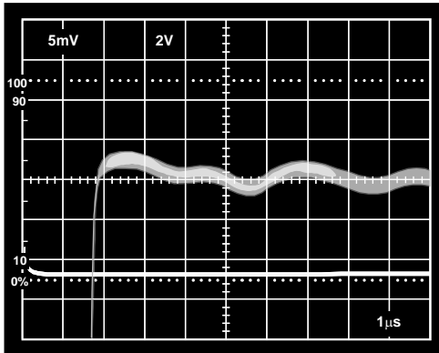
Figure 47. Positive Slope Settling Time
