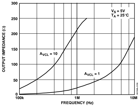
Figure 25. Output Impedance vs. Frequency
