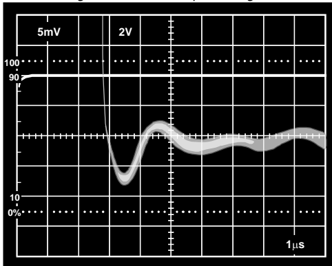
Figure 48. Negative Slope Settling Time
