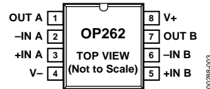
Figure 2. 8-Lead Narrow-Body SOIC (S Suffix)
