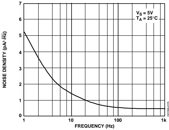
Figure 24. Current Noise Density vs. Frequency
