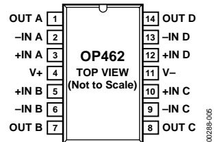
Figure 4. 14-Lead Narrow-Body SOIC (S Suffix)
