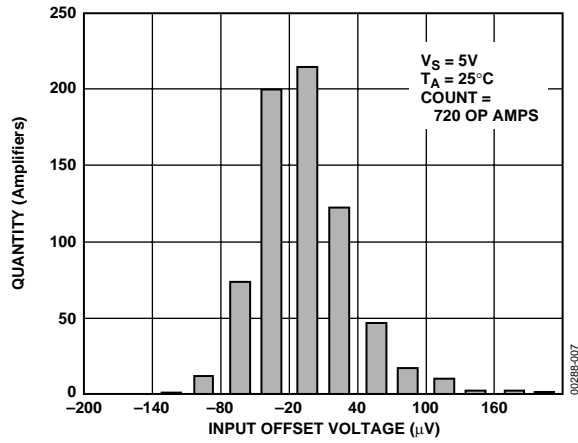
Figure 6. OP462 Input Offset Voltage Distribution
