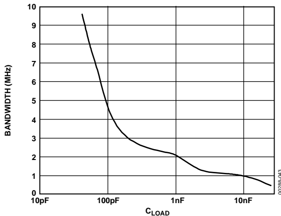
Figure 42. Unity-Gain Bandwidth vs. C_{LOAD}
