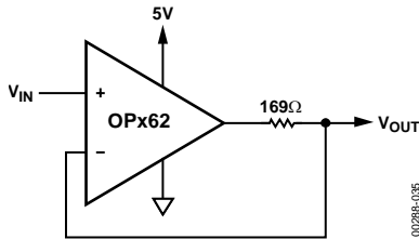
Figure 34. Output Short-Circuit Protection
