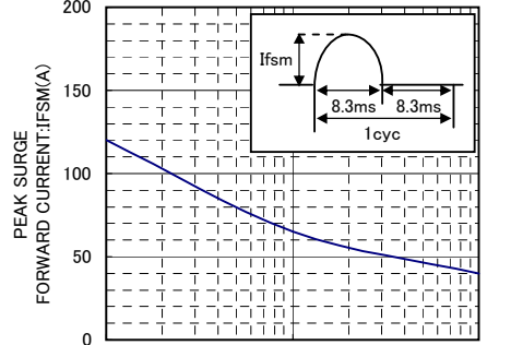
NUMBER OF CYCLES IFSM-CYCLE CHARACTERISTICS
