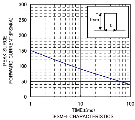
IFSM-t CHARACTERISTICS
