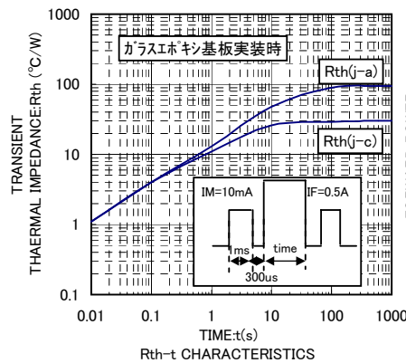
Rth-t CHARACTERISTICS
