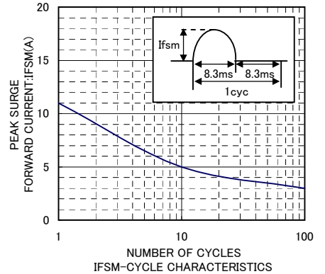
IFSM-CYCLE CHARACTERISTICS
