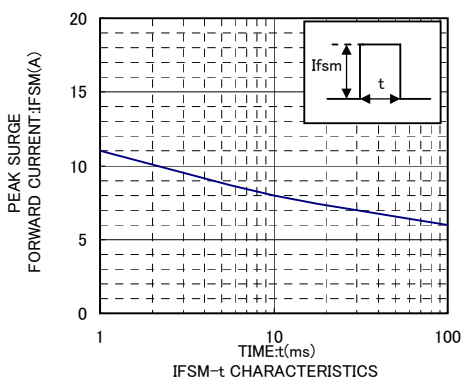
IFSM-t CHARACTERISTICS
