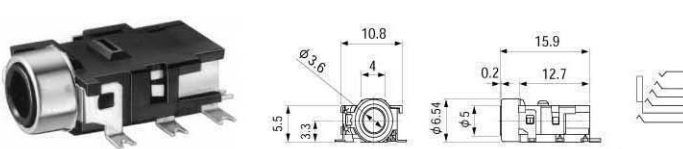
No.MJ-354W-S2 3.5MM STEREO JACK FOR P.C. W/SHIELD HOUSING
