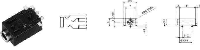
No.MJ-2-348A0 (φ2.5) With Metal Sleeve No.MJ-2-348B0 (φ2.5) Without Metal Sleeve SUB-MINIATURE STEREO JACK
