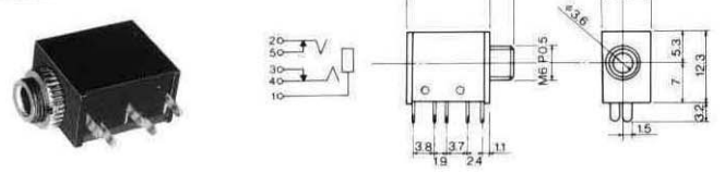
No.MX-238A0 (φ3.5) STEREO
