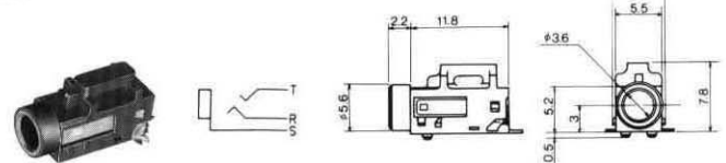
No.MX-238A0 (φ3.5) STEREO
