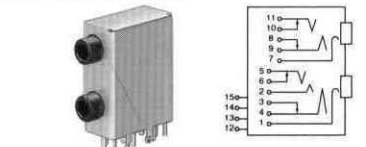
No.MJ-653 3.5MM DOUBLE STEREO JACK FOR P.C. W/FULL SHIELD HOUSING
