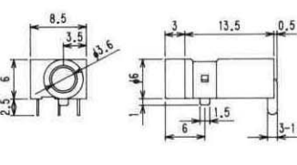
No.MJ-653 3.5MM DOUBLE STEREO JACK FOR P.C. W/FULL SHIELD HOUSING
