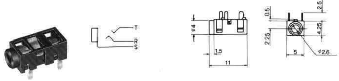
No.M02-641A0 (φ2.5) STEREO
