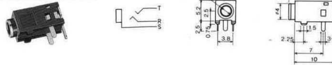
No.MJ-2-348A0 (φ2.5) With Metal Sleeve No.MJ-2-348B0 (φ2.5) Without Metal Sleeve SUB-MINIATURE STEREO JACK
