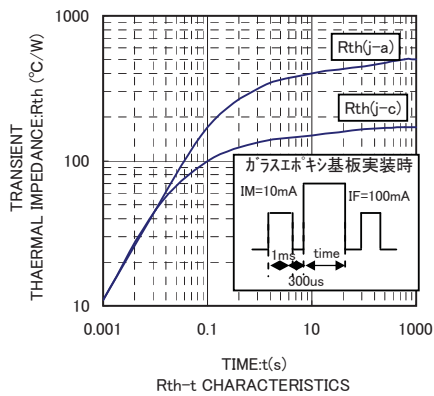
Rth-t CHARACTERISTICS
