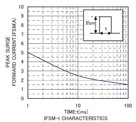
IFSM-t CHARACTERISTICS
