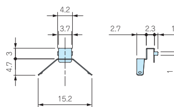
CST-2450P
