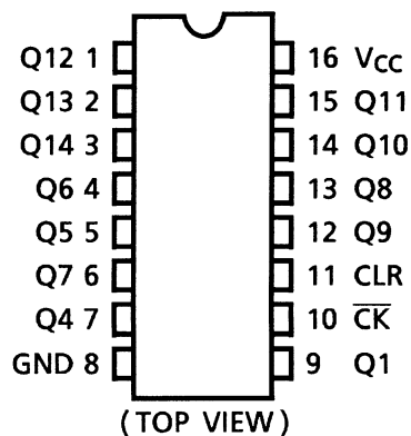
TC74HC4020A
