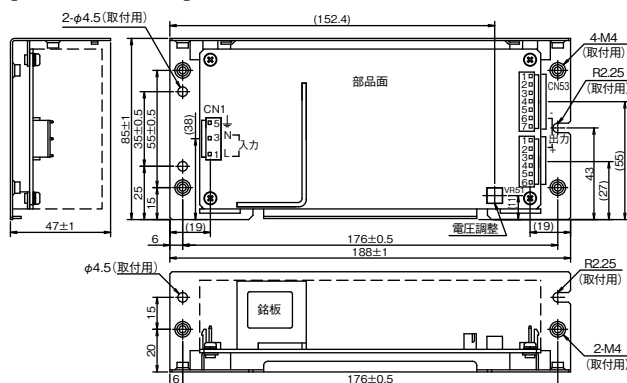
[ZWS150BAF/L]
