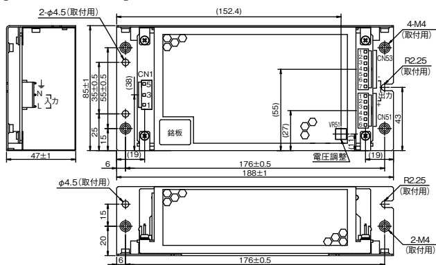
[ZWS150BAF/A]
