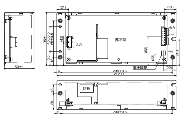
[ZWS300BAF/L]
