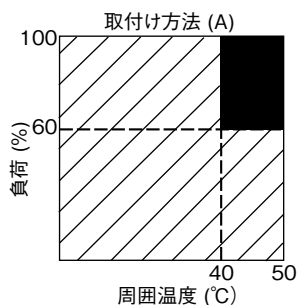
ZWS300BAF-24, 36, 48
