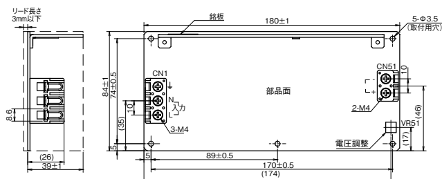
[ZWS300BAF/T]
