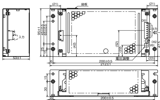
[ZWS300BAF/A]
