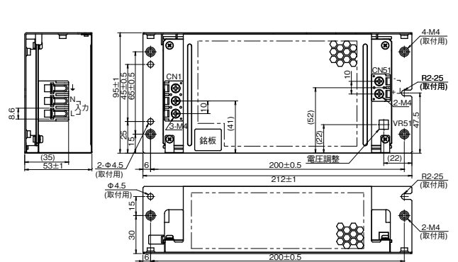
[ZWS300BAF/TA]
