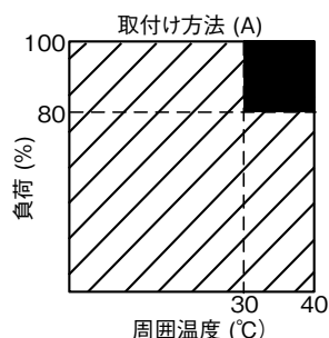
ZWS300BAF-12, 15
