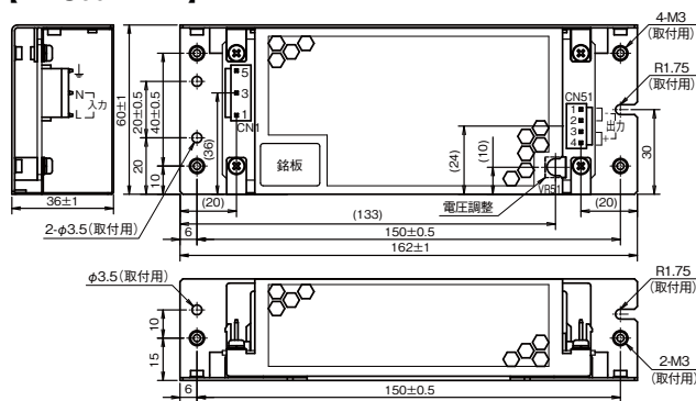
[ZWS50BAF/A]
