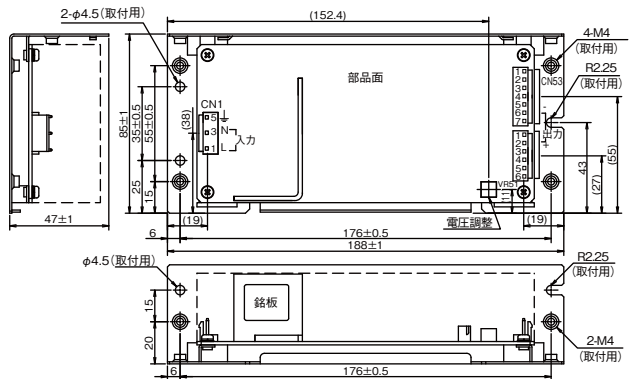
[ZWS150BAF/L]
