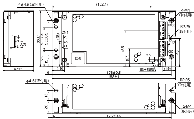
[ZWS150BAF/A]
