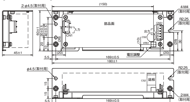
[ZWS75BAF/L]
