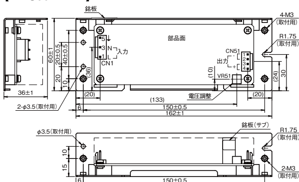
[ZWS50BAF/L]
