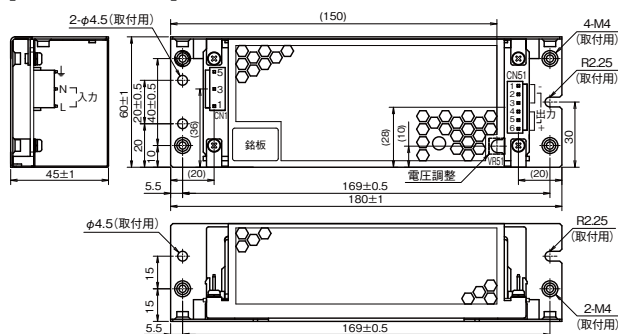
[ZWS75BAF/A]
