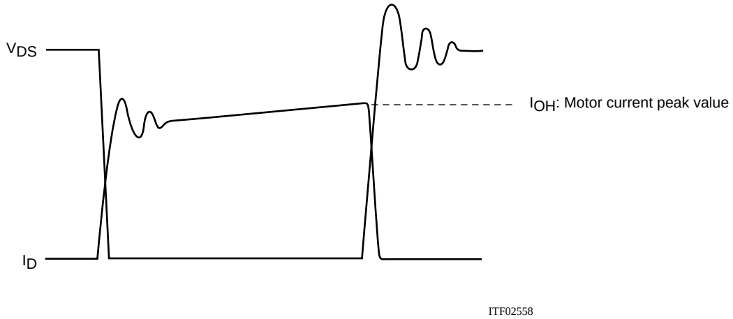
Figure 2 Output Current, I_D , and Voltage, V_{DS} , Waveforms 2 of the STK672-4** Series when Driving a 2-Phase Stepping Motor with Constant Current Chopping
