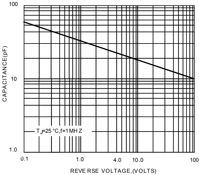
FIG.3-TYPICAL JUNCTION CAPACITANCE
