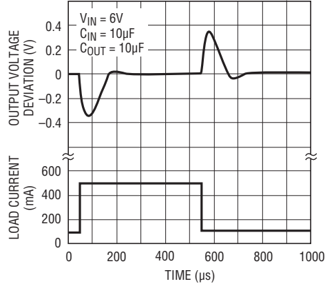
LT1763-5の過渡応答 C_{BYP} = 0
