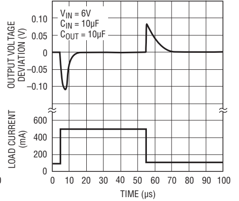
LT1763-5の過渡応答 C_{BYP} = 0.01\mu F
