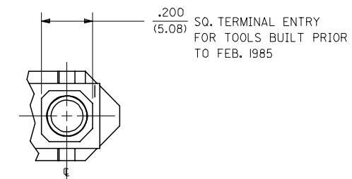
DETAIL "I"
