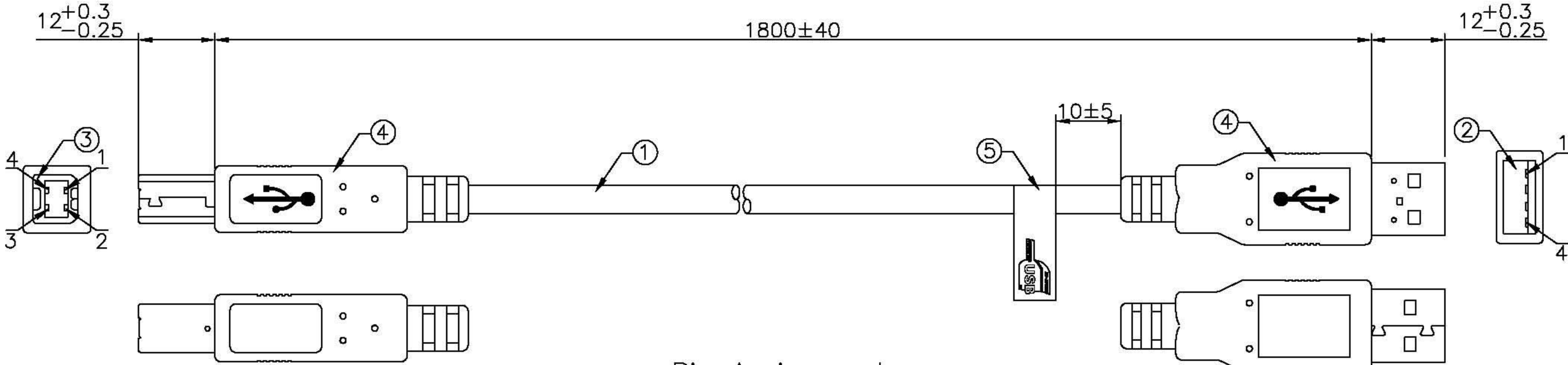
Conn.2 USB("A") Male
