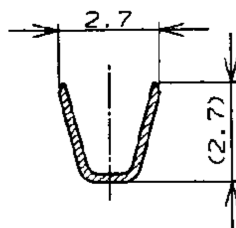
断面 "A"- "A" SECT
