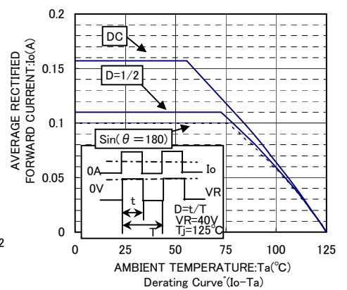
Derating Curve ( I_o - T_a )
