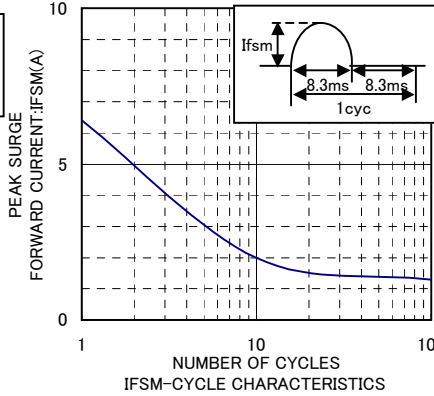
IFSM-CYCLE CHARACTERISTICS
