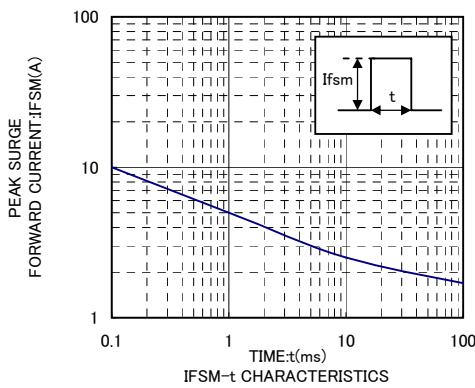
IFSM-t CHARACTERISTICS
