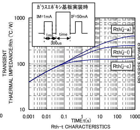
Rth-t CHARACTERISTICS
