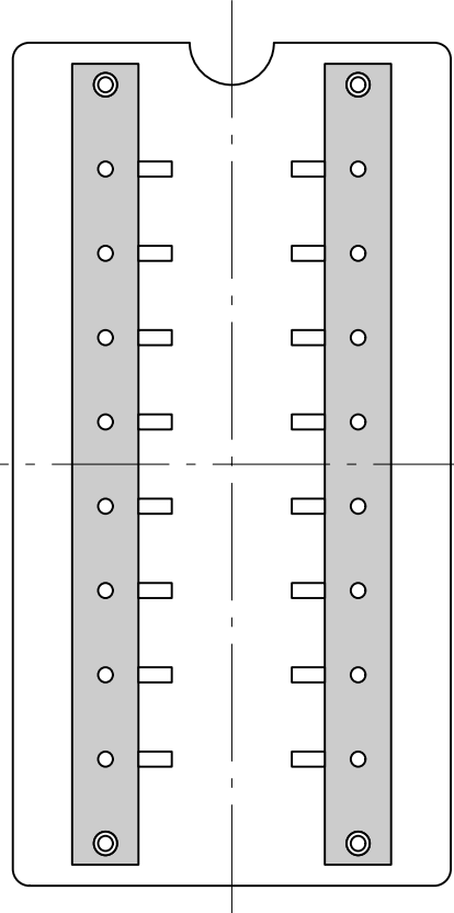
Size of SOP pads Scale 3:1
