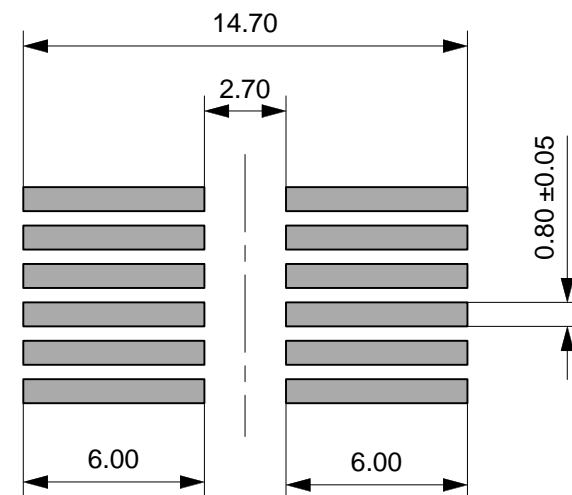
Size of SOP pad Scale 4:1
