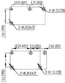
Drilling Plan孔位图 (Bottom View底视图)
