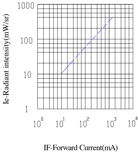
Fig.5 Relative Intensity vs. Forward Current
