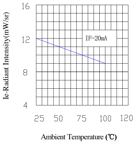
Fig.7 Relative Intensity vs. Ambient Temperature (°C)
