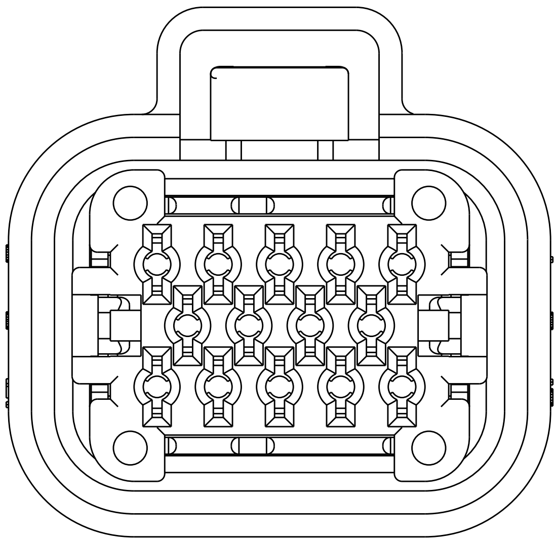
BOTTOM VIEW WITH LOCKING WEDGE
