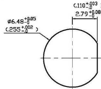
MOUNTING HOLE
