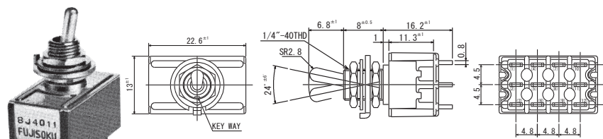
Terminal numbers are not shown on the switch.
