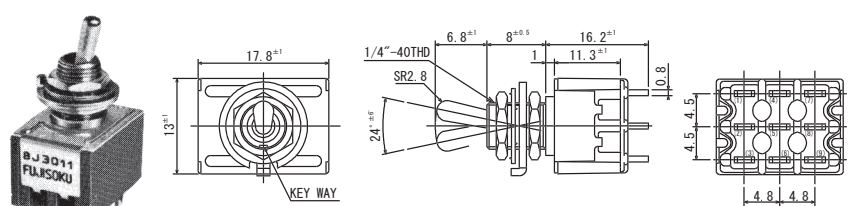
Terminal numbers are not shown on the switch.
