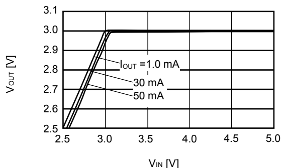
S-1200B30 ( T_a=+25^\circ\text{C} )
