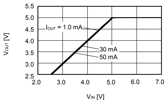
S-1200B50 ( T_a=+25^\circ\text{C} )
