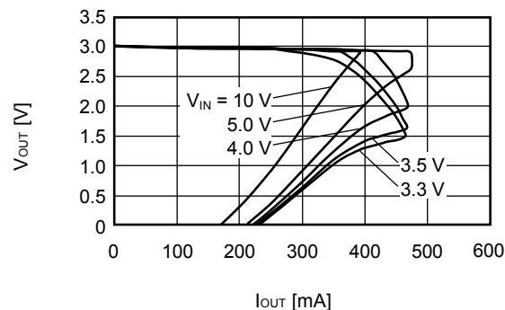
S-1200B30 ( T_a=+25^\circ\text{C} )
