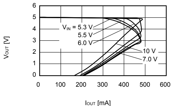
S-1200B50 ( T_a=+25^\circ\text{C} )
