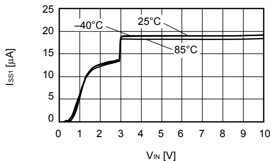
S-1200B30
