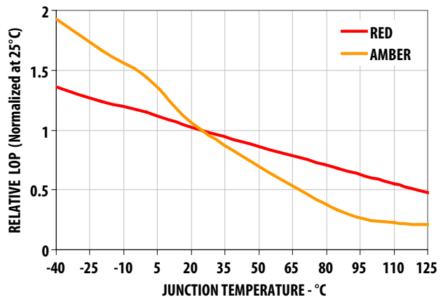
Figure 6. Relative LOP (Normalized at 25^\circ\text{C} ) vs. junction temperature for AllnGaP
