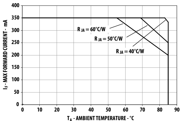
Figure 5. Maximum forward current vs. ambient temperature for AllnGaP Derated based on T_{j,MAX} = 125^\circ\text{C} , R_{\theta_{jA}} = 40^\circ\text{C/W} / 50^\circ\text{C/W} and 60^\circ\text{C/W}
