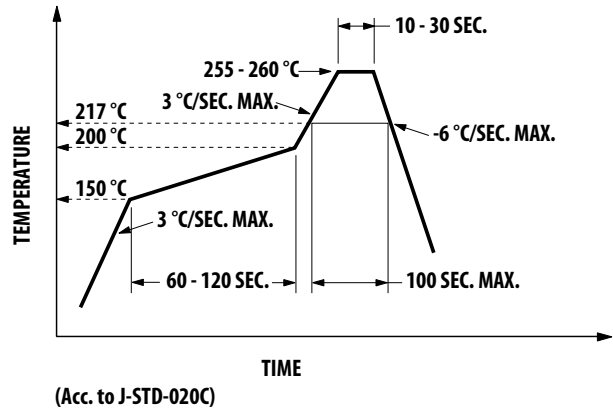
Figure 14. Recommended reflow soldering profile (Acc. to J-STD-020C)
