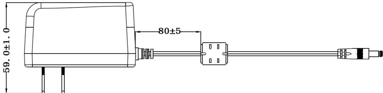
SIDE VIEW
