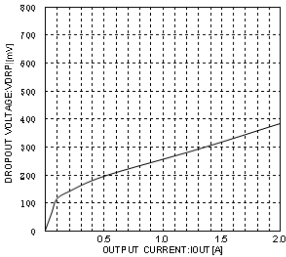
Fig.17 Input/Output Voltage Difference I_{OUT}-\Delta V_d Characteristics ( V_{CC}=4.75V )
