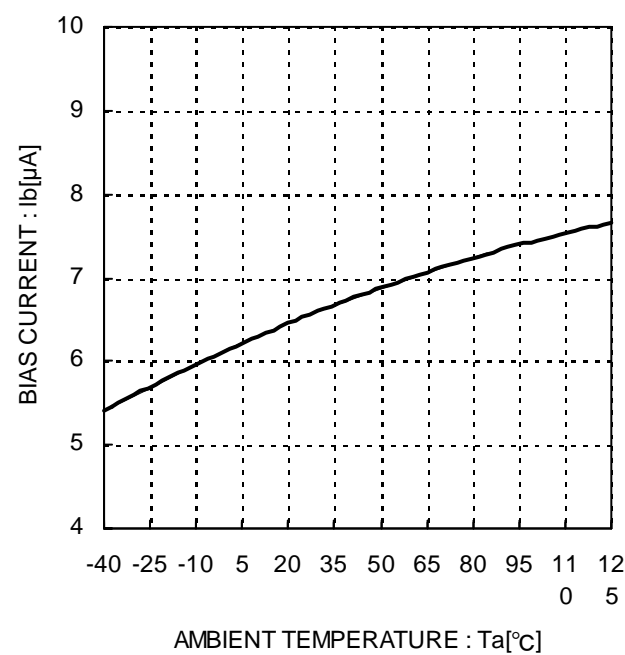
Figure 24. Bias current vs. Temperature
