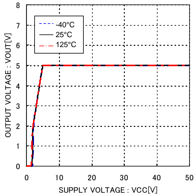
Figure 17. Output voltage vs. Supply voltage IOUT=100mA
