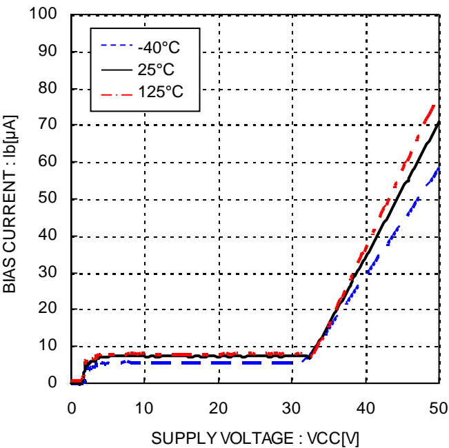
Figure 15. Bias current
