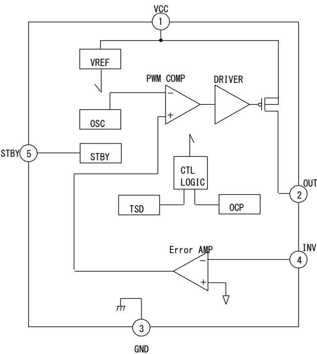
Figure 2. Block Diagram
