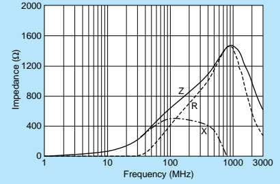
BLM15HD601SN1
