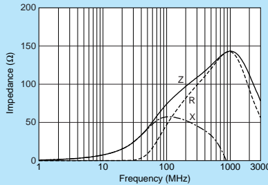
BLA2ABD750SN4
