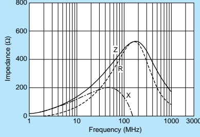
BLM21AG471SN1
