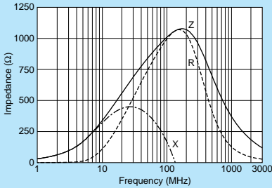
BLA2AAG102SN4
