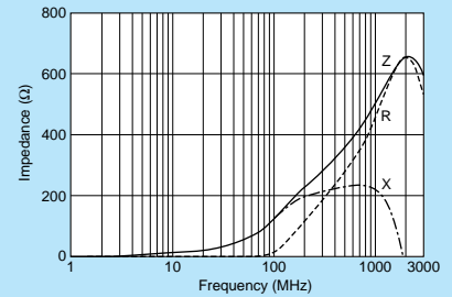
BLM15HB121SN1
