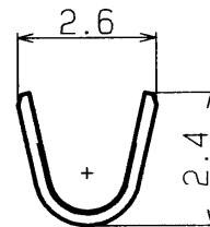
WIRE BARREL
