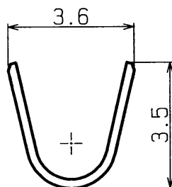
INSULATION BARREL
