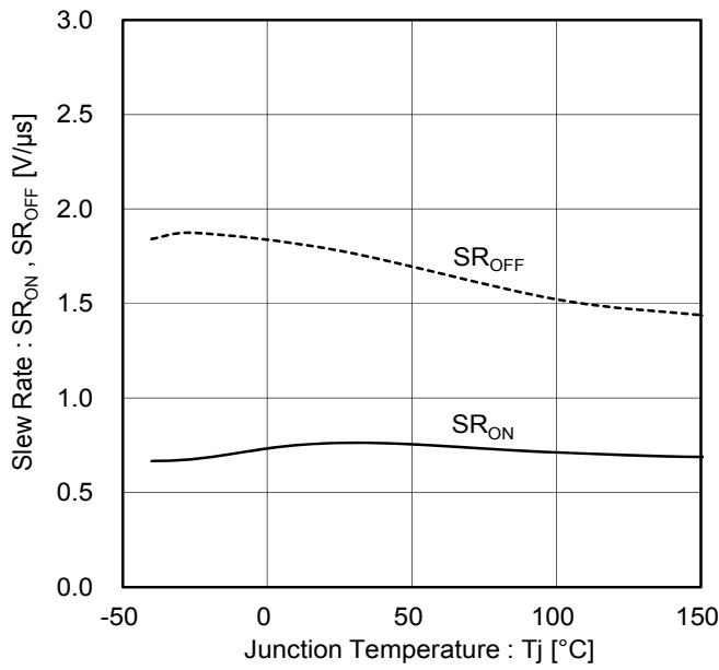
Figure 17. Slew Rate vs. Temperature
