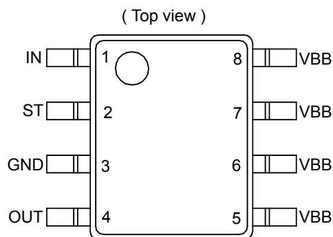
Figure 2. Pin Configurations
