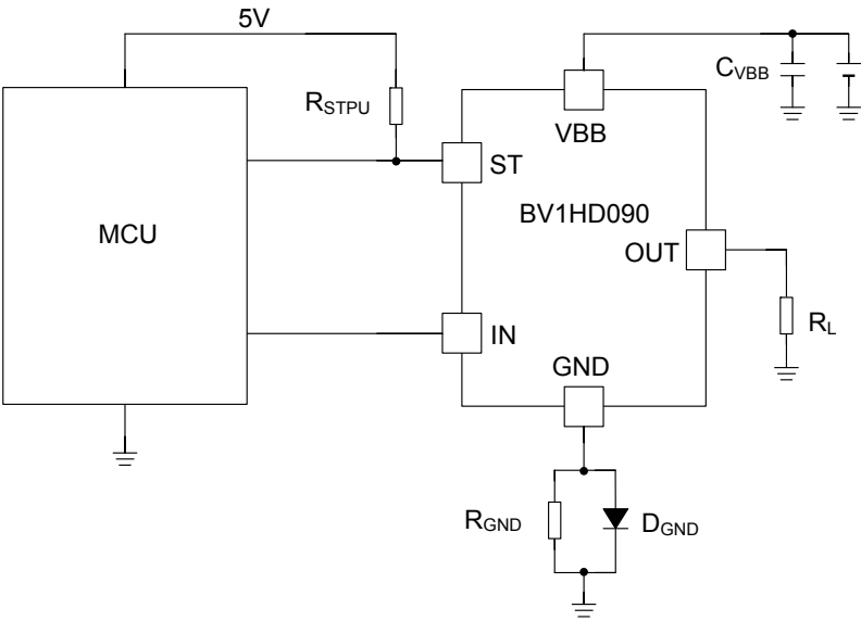
Figure 40. Application Circuits
