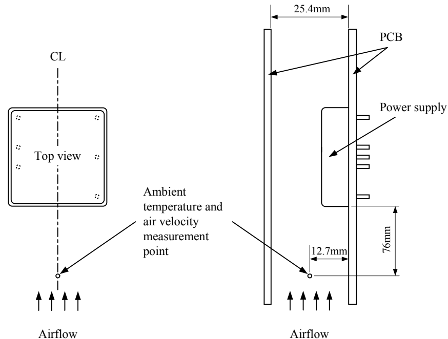
Fig.7-2 Output Current VS Ambient Temperature Measurement Method (for forced cooling)
