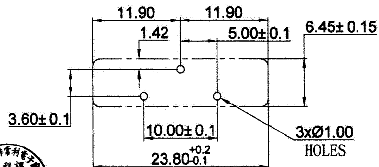
PCB MOUNTING LAYOUT
