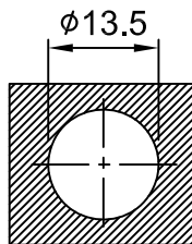
PANEL APERTURE
